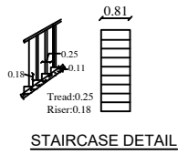
STAIRCASE DETAIL
