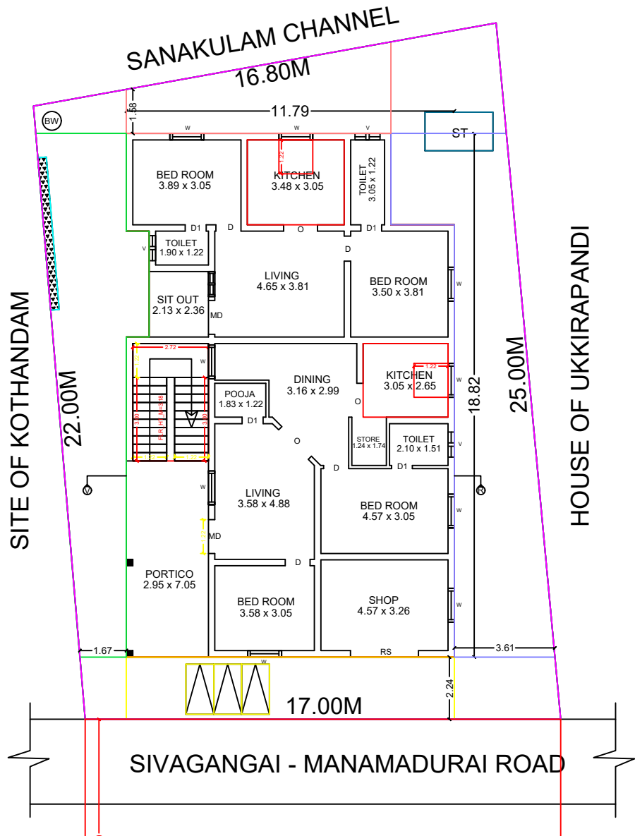
M EXISTING FLOOR PLAN
