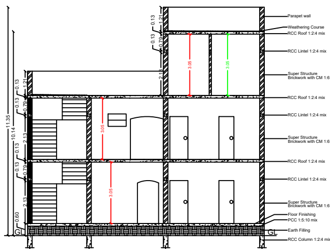
SECTION ON "VR"
