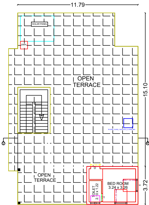
PROPOSED SECOND & TERRACE FLOOR PLAN
