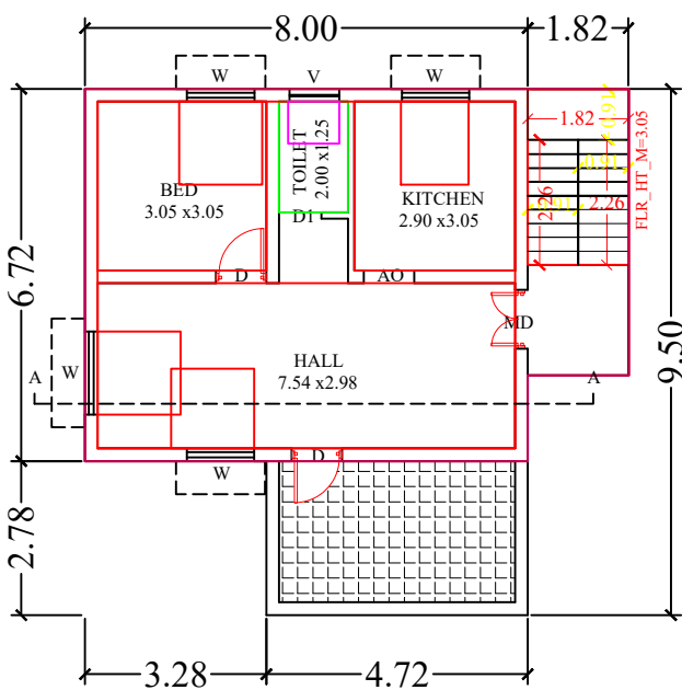
FIRST FLOOR PLAN (PROPOSED BUILDING)
