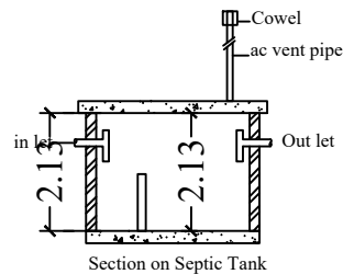
Section on Septic Tank
