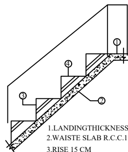
SECTIONS OF STAIR CASE
