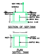
PLAN SEPTIC TANK
