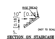
SECTION ON STAIRCASE (NOT TO SCALE)
