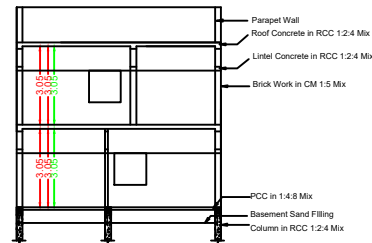
Section RR
