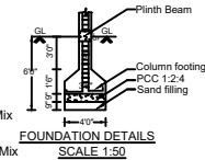
FOUNDATION DETAILS SCALE 1:50
