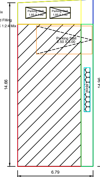
Site Plan
