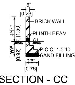
SECTION - CC
