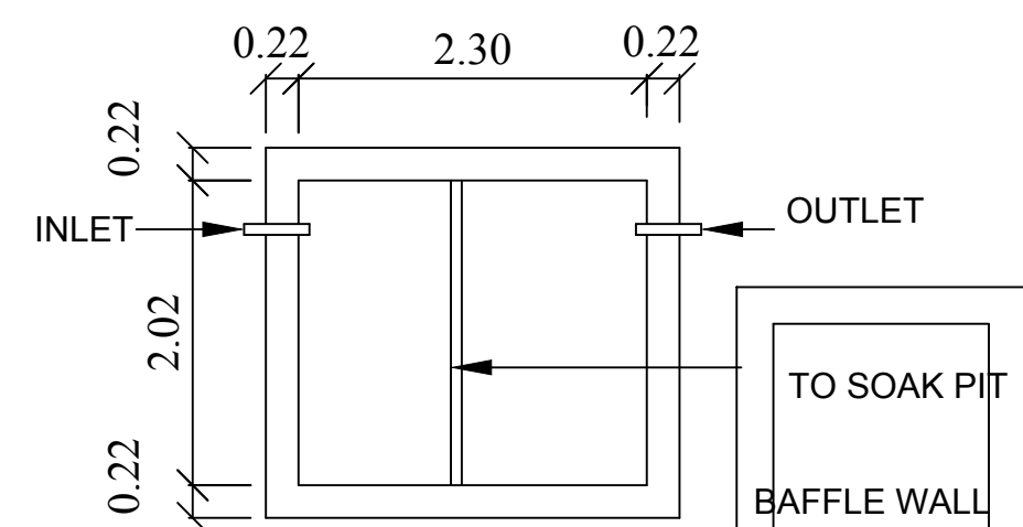
PLAN SEPTIC. TANK
