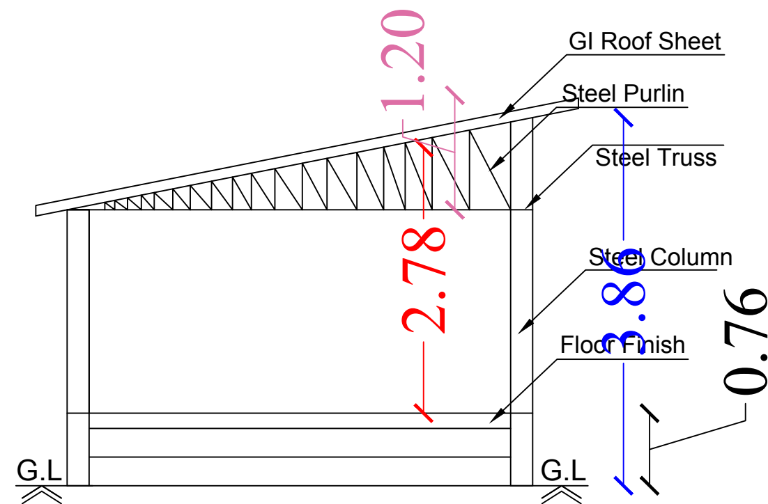
Section on-"AA"
