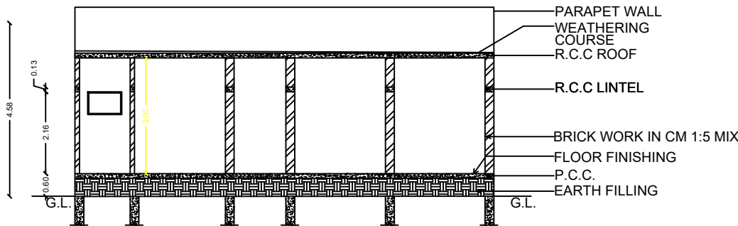
SECTION ON "VR"
