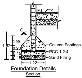
Foundation Details Section
