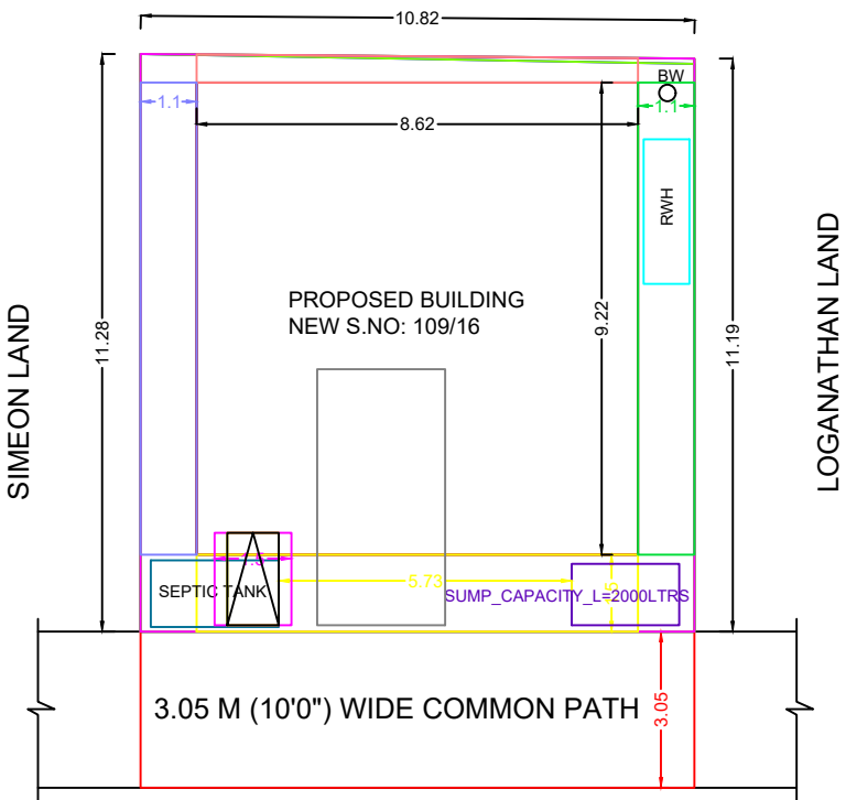
SITE PLAN
