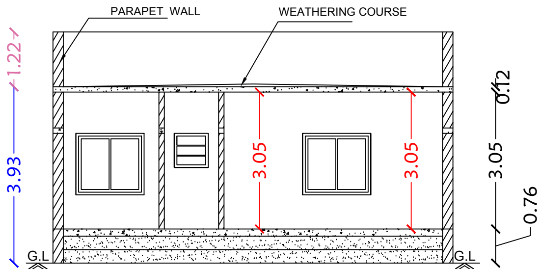
Section on-"AA"
