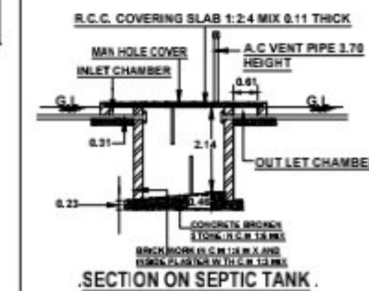
SECTION ON SEPTIC TANK.
