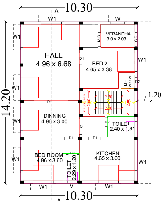
PRO.GROUND FLOOR
