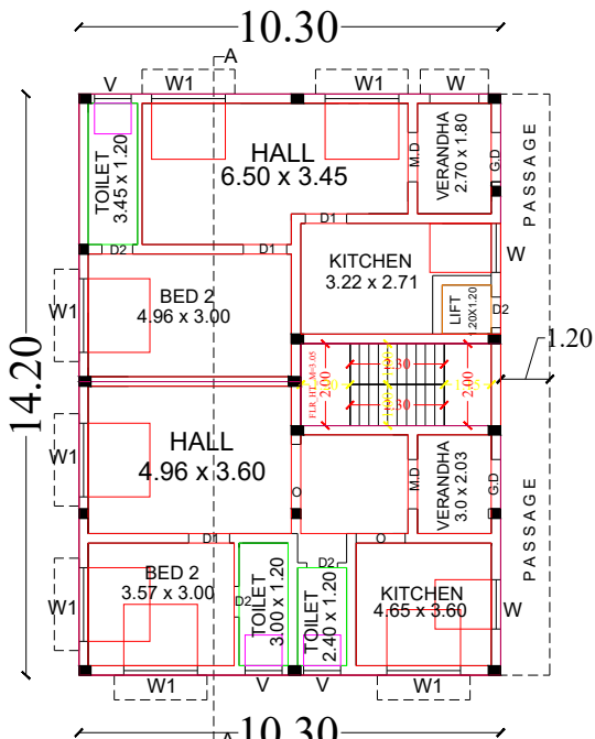
PRO.SECOND FLOOR
