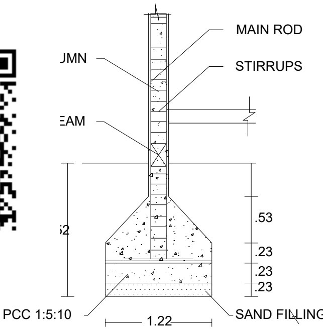
COLUMN DETAILS
