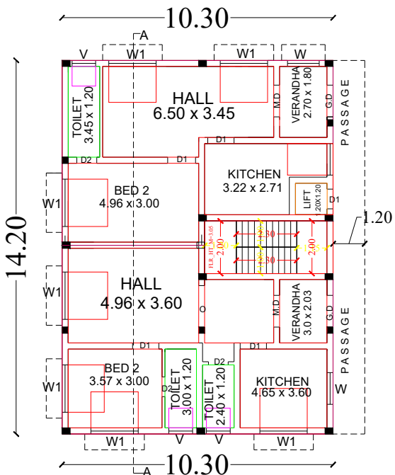
PRO.FIRST FLOOR
