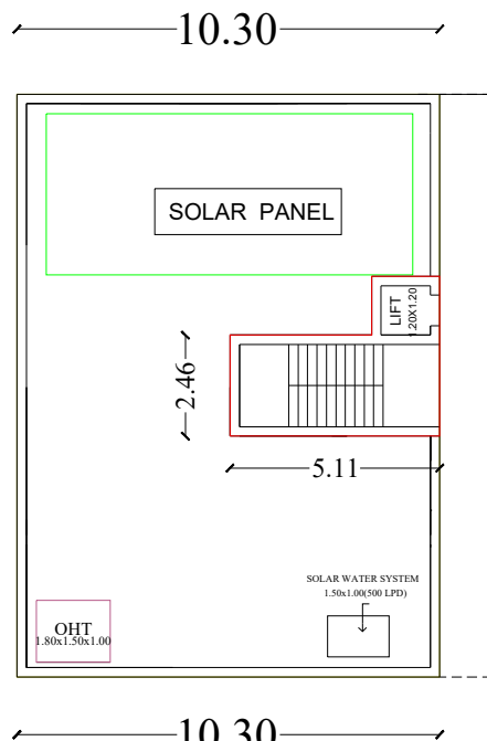
TERRACE FLOOR
