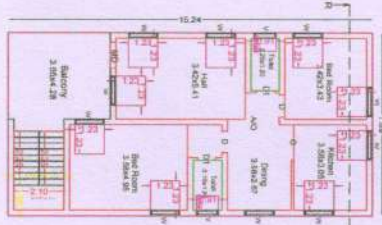
Pro. First Floor Plan
