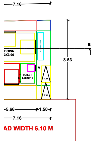
PRO. GROUND FLOOR PLAN
