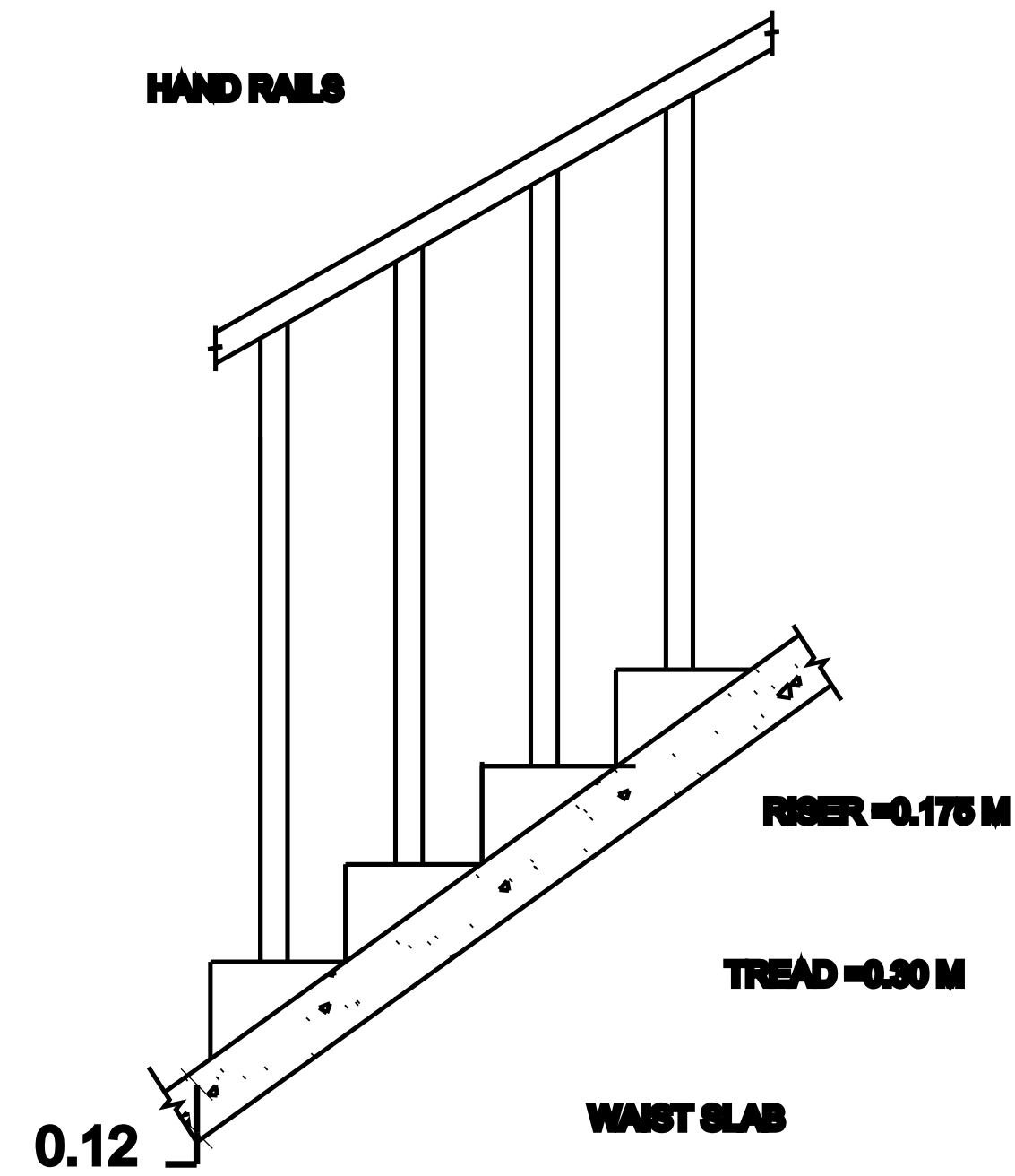
STAIR CASE DETAILS
