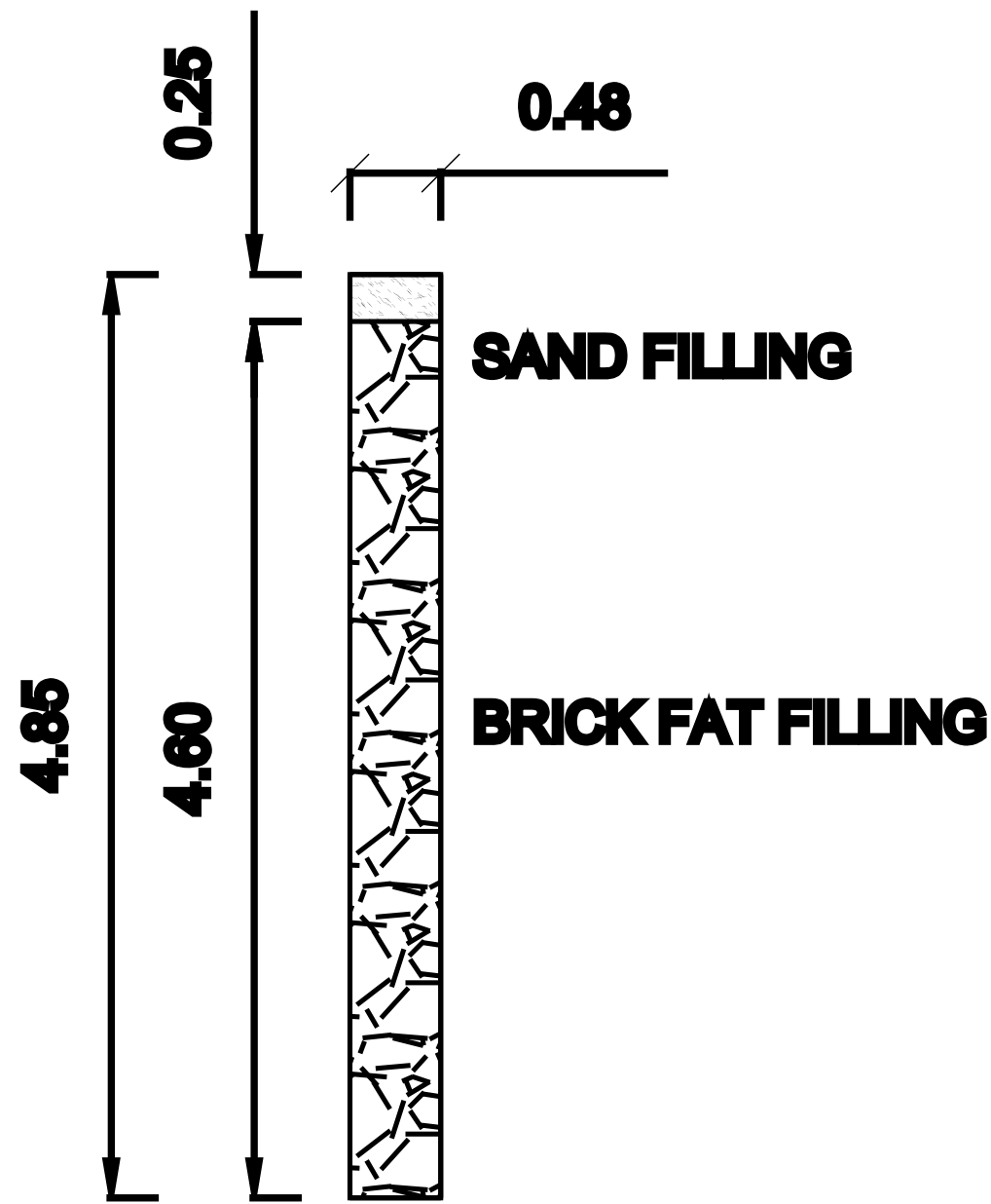
DETAILS OF PERCULATION PIT
