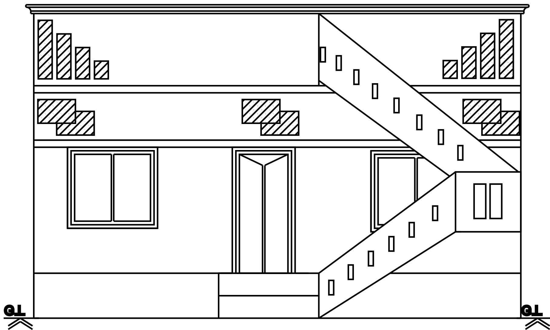
Front Elevation
