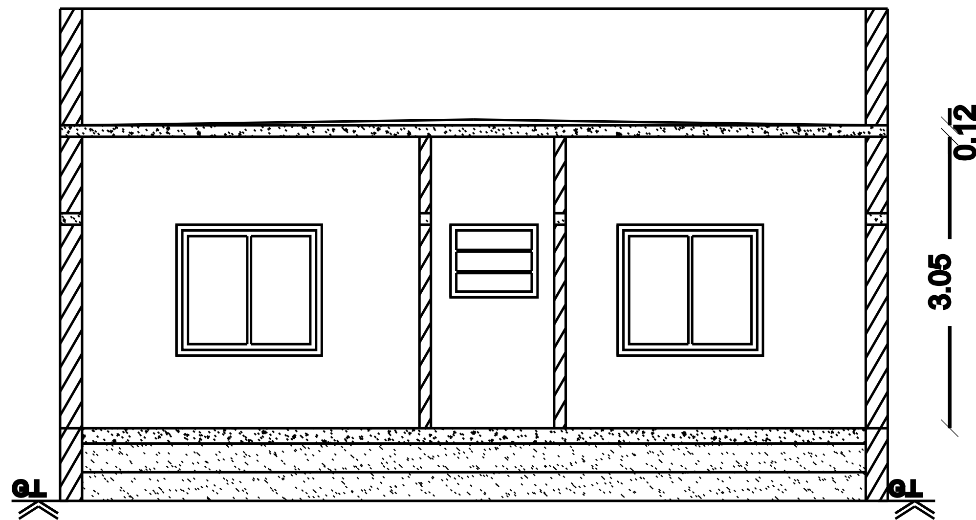
Section on-"AA"
