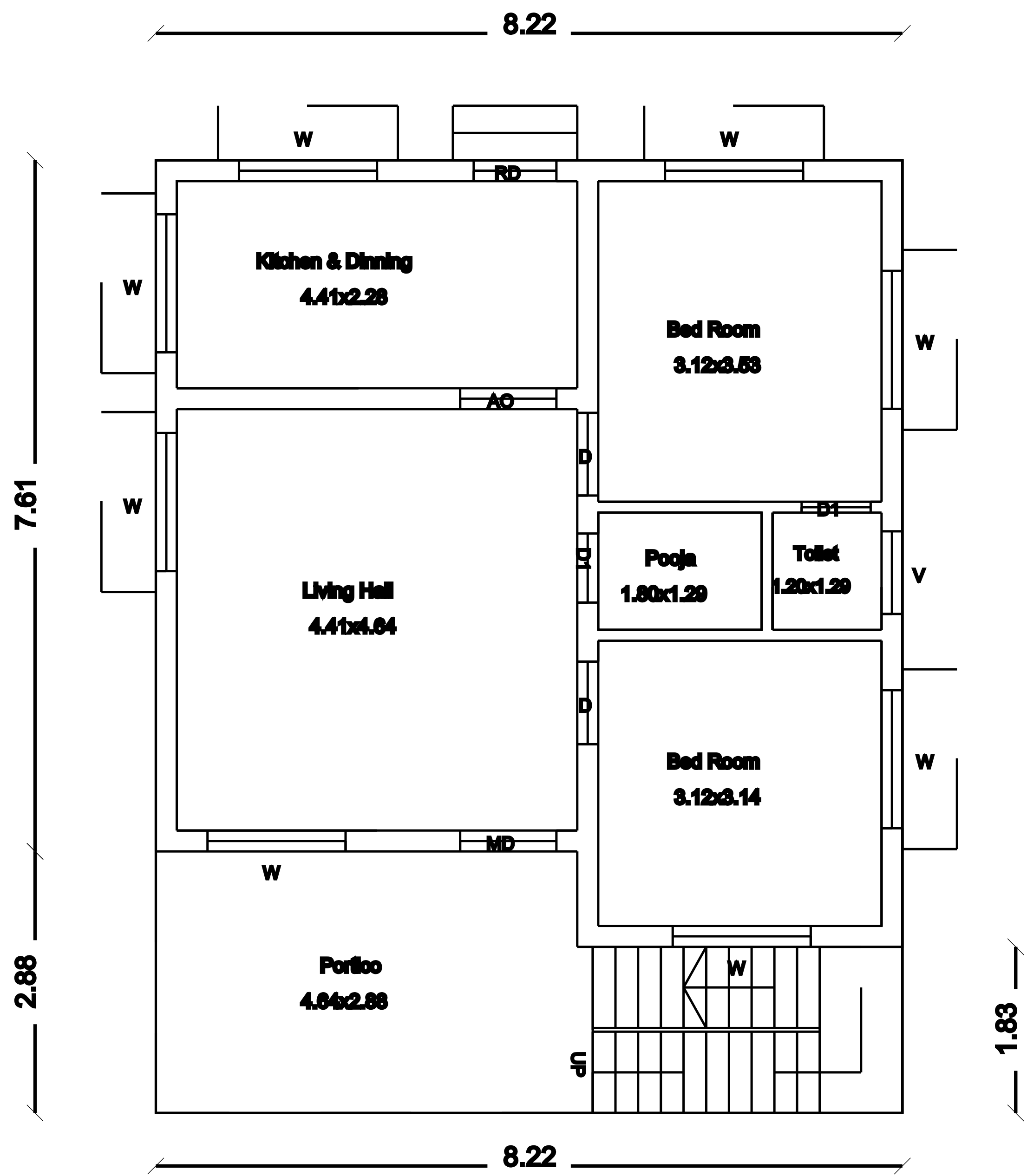
Ground Floor
