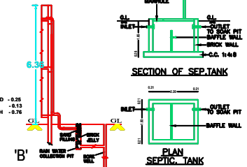
RAIN WATER HARVESTING SYSTEM RWPH_CAPACITY_1=100LITRES
