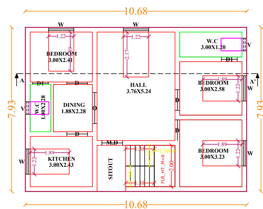
PRO GROUND FLOOR
