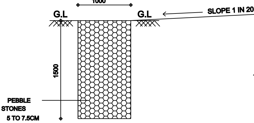
SECTION OF PEBBLE TRENCH
