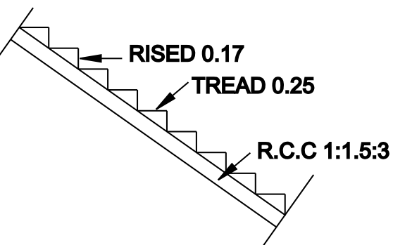
STAIRCASE DETAILS
