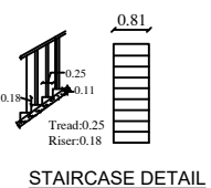
STAIRCASE DETAIL
