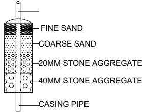
DETAILS OF RAIN WATER HARVESTING STRUCTURES
