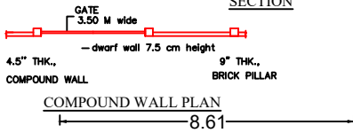
COMPOUND WALL DETAILS
