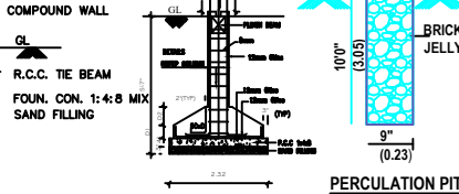
FOUNDATION DETAILS
