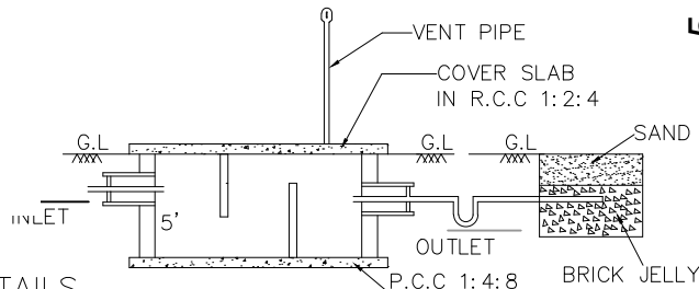
SECTION-AB
