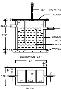
SEPTIC TANK DETAILS (NOT TO SCALE)
