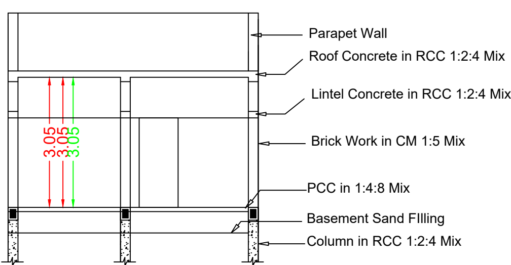
Section RR
