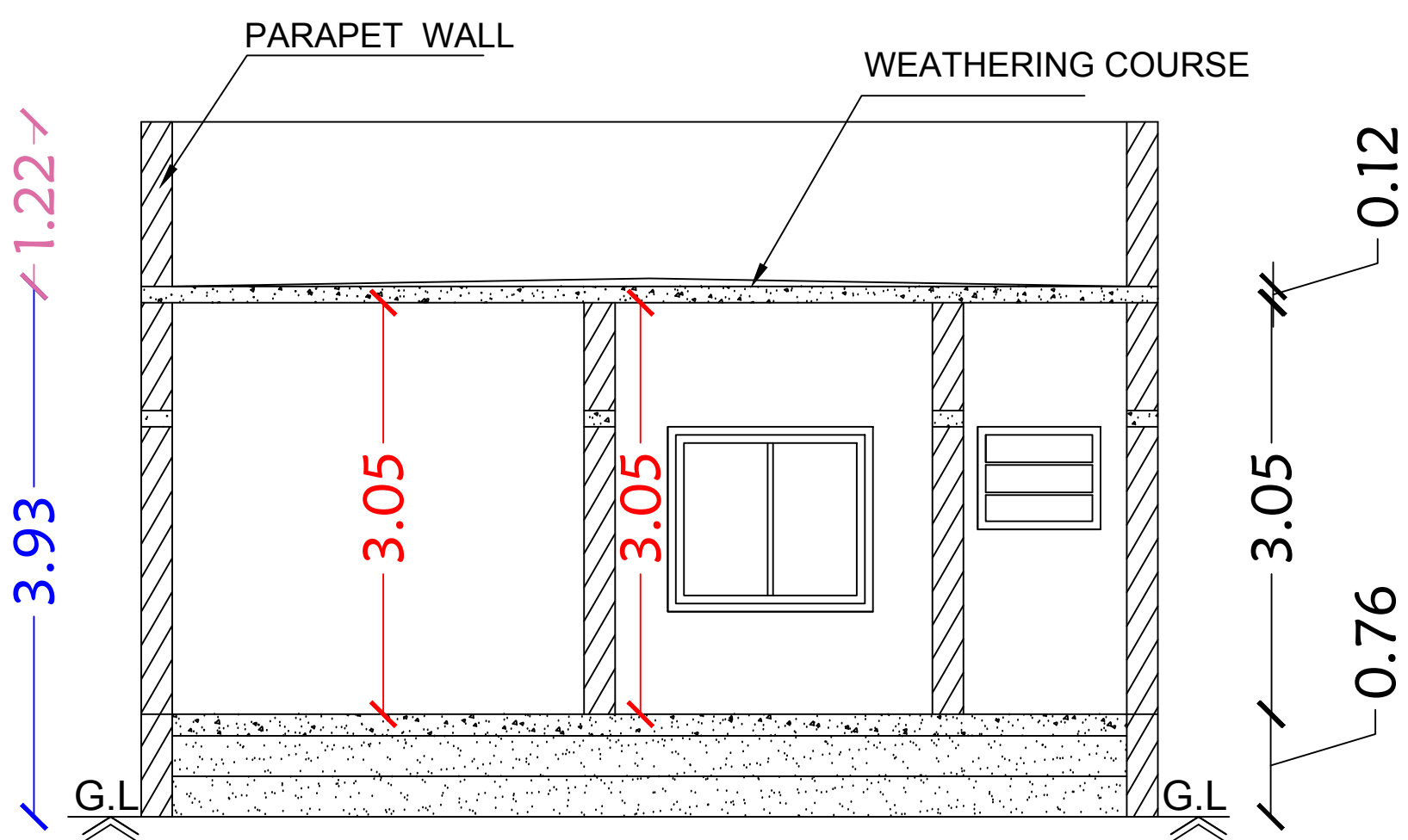
Section on-"AA"
