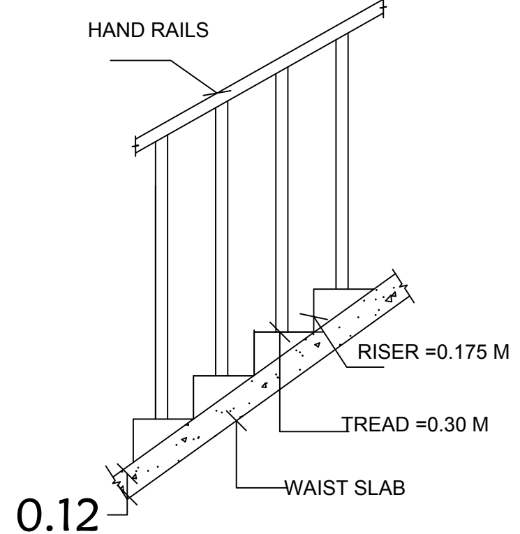
STAIR CASE DETAILS
