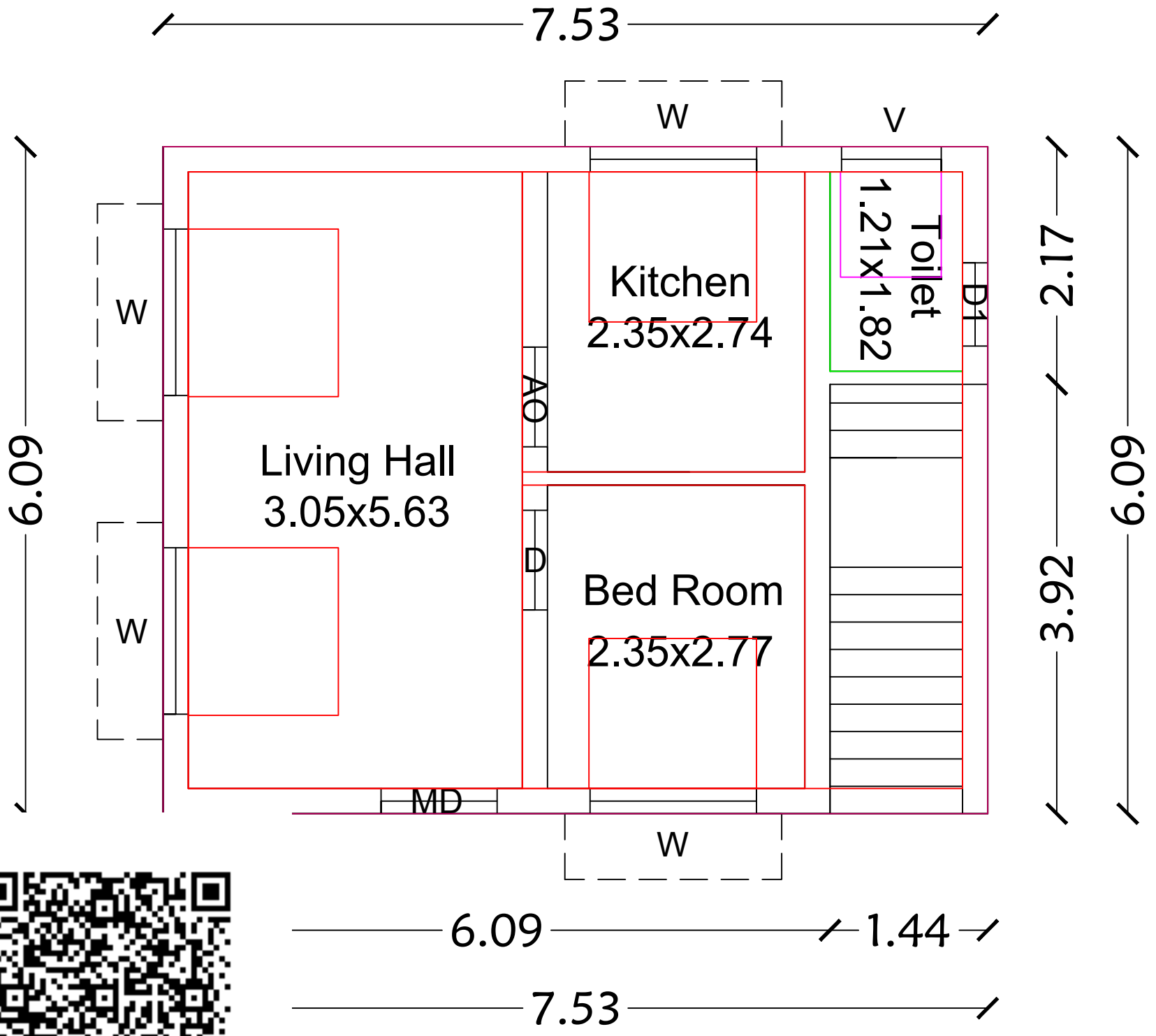
Ground Floor
