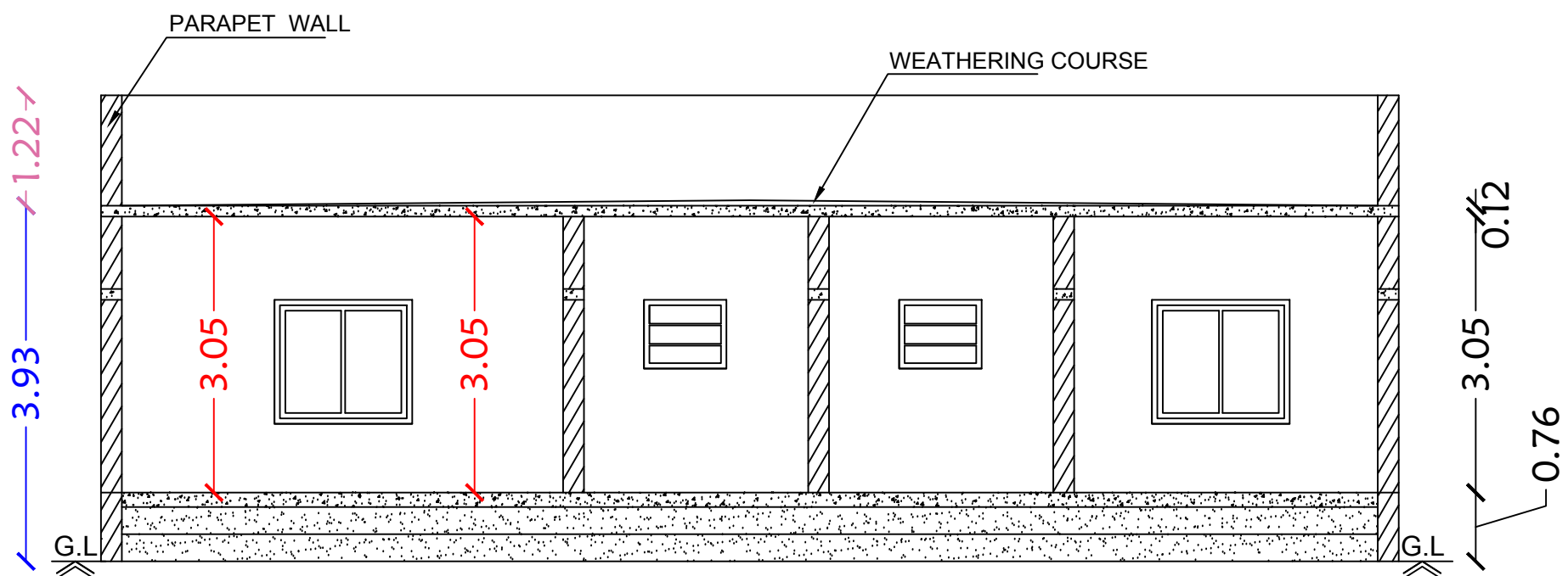
Section on-"AA"
