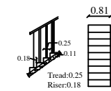
STAIRCASE DETAIL
