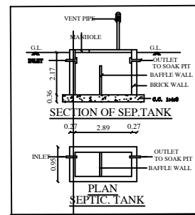
CUT SECTION ON AA
