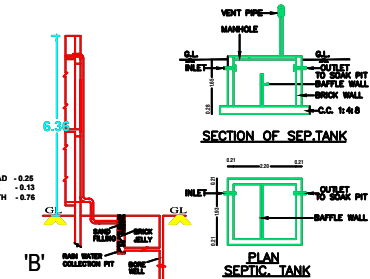
RAIN WATER HARVESTING SYSTEM RWHS_CAPACITY_1=1000LTRS
