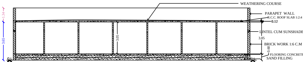
Section on-"AA"
