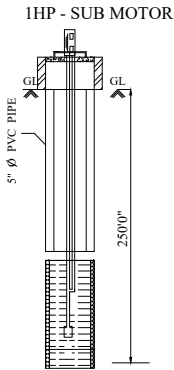
BOREWELL DETAILS
