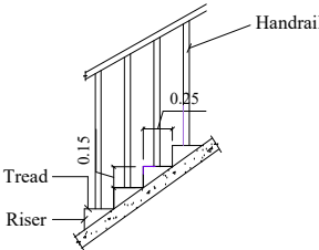
STAIRCASE DETAIL
