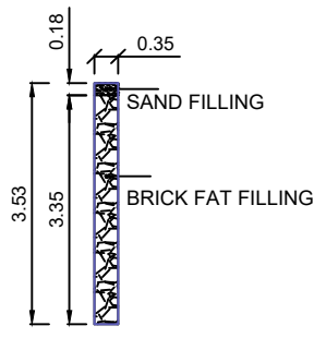
PERCULATION PIT
