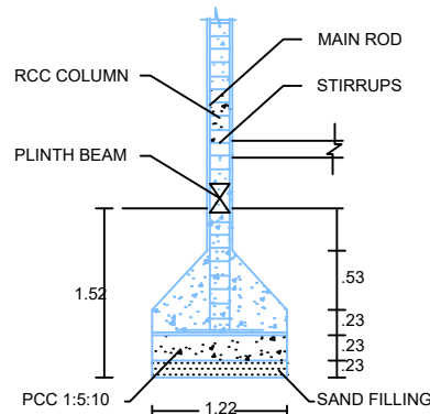
COLUMN DETAILS
