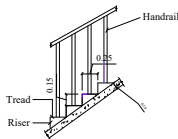
STAIRCASE DETAIL
