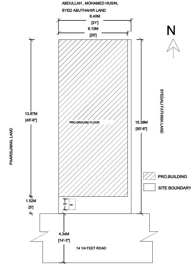
SITE PLAN
