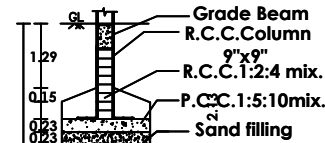
COLUMN DETAILS
