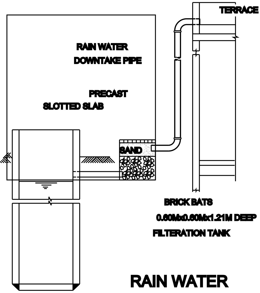
RAIN WATER HARVESTING SYSTEM
