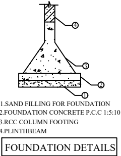
FOUNDATION DETAILS
