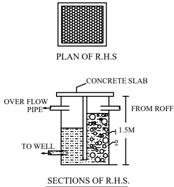
SECTIONS OF R.H.S.
