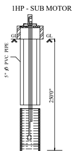
BOREWELL DETAILS
