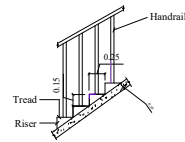
STAIRCASE DETAIL
