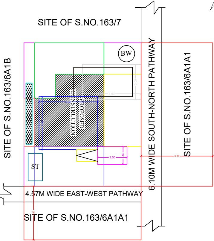
SITE PLAN
