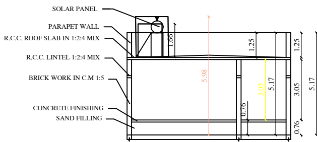
CUT SECTION ON AA
