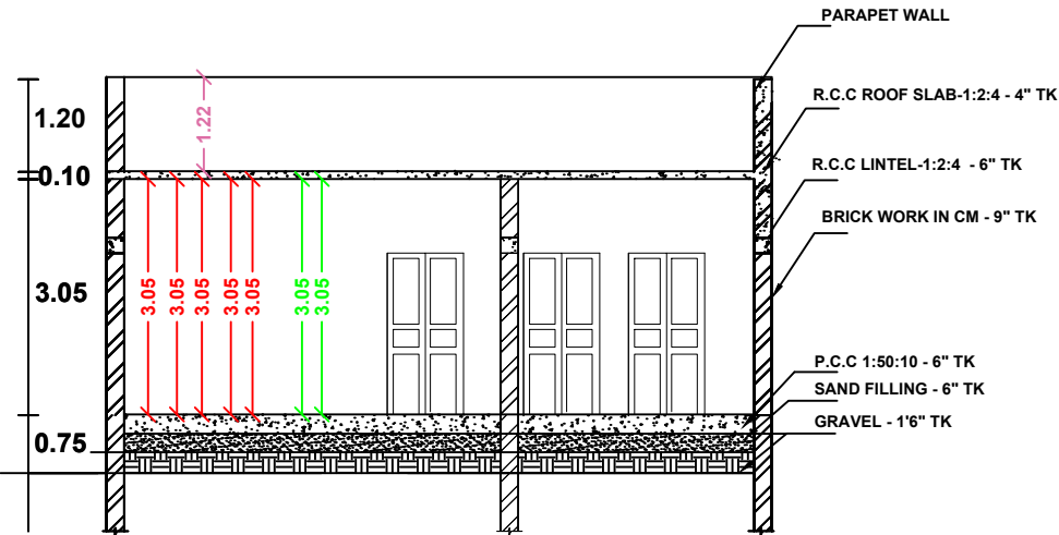
SECTION AB
