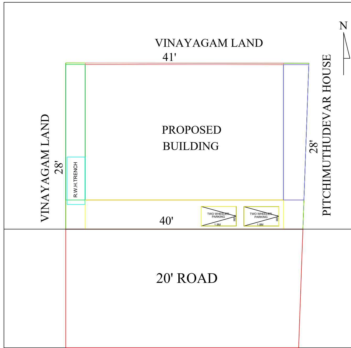
SITE PLAN
