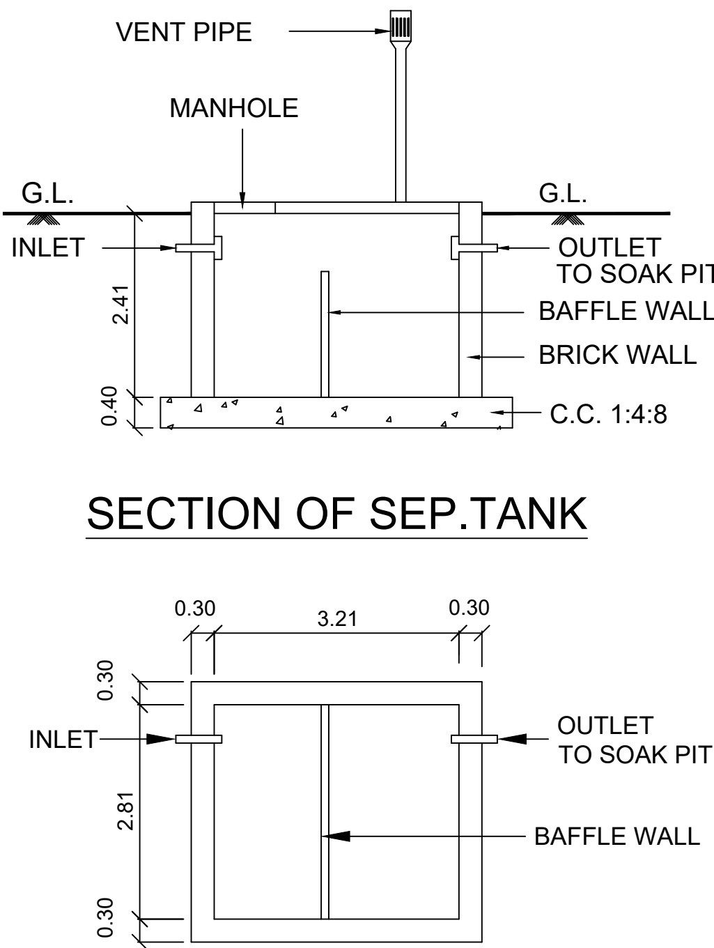
SEPTIC. TANK
