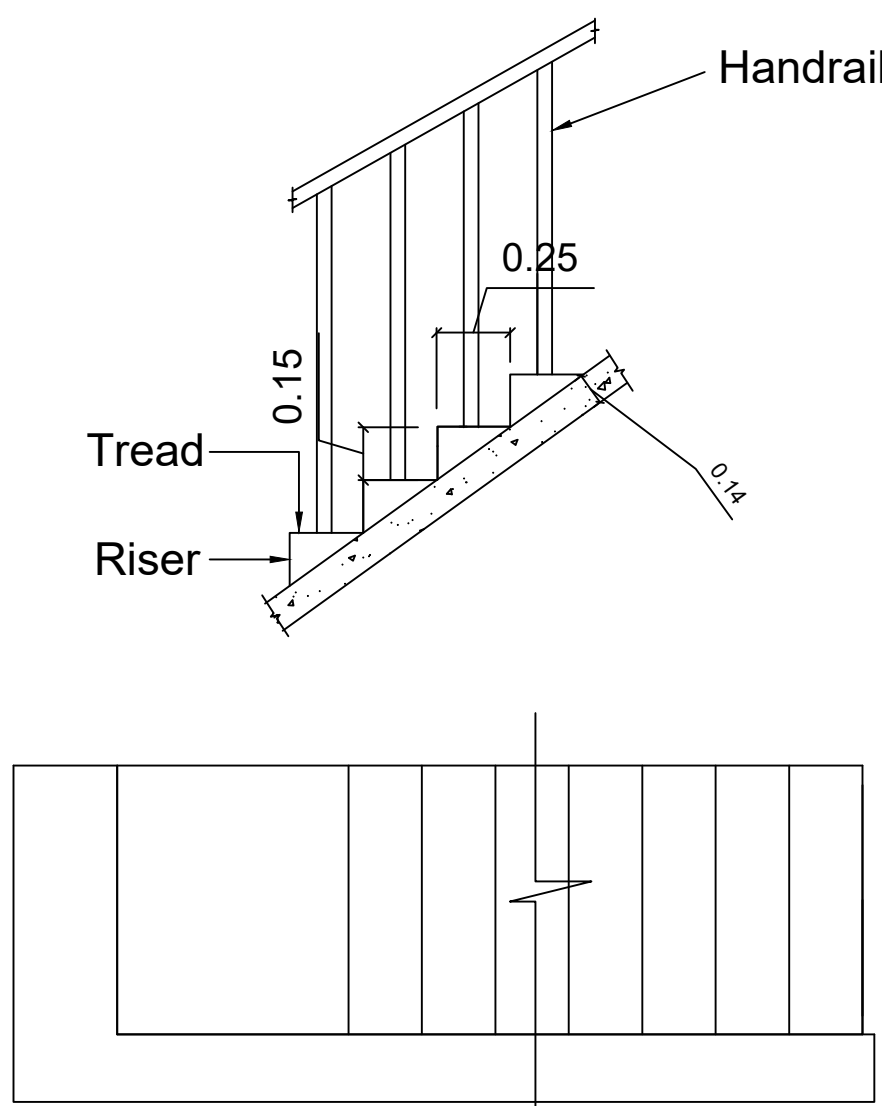
STAIRCASE DETAIL
