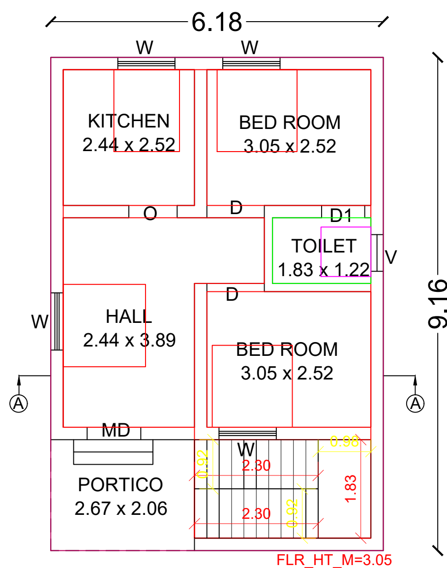
ROUND FLOOR PLAN
