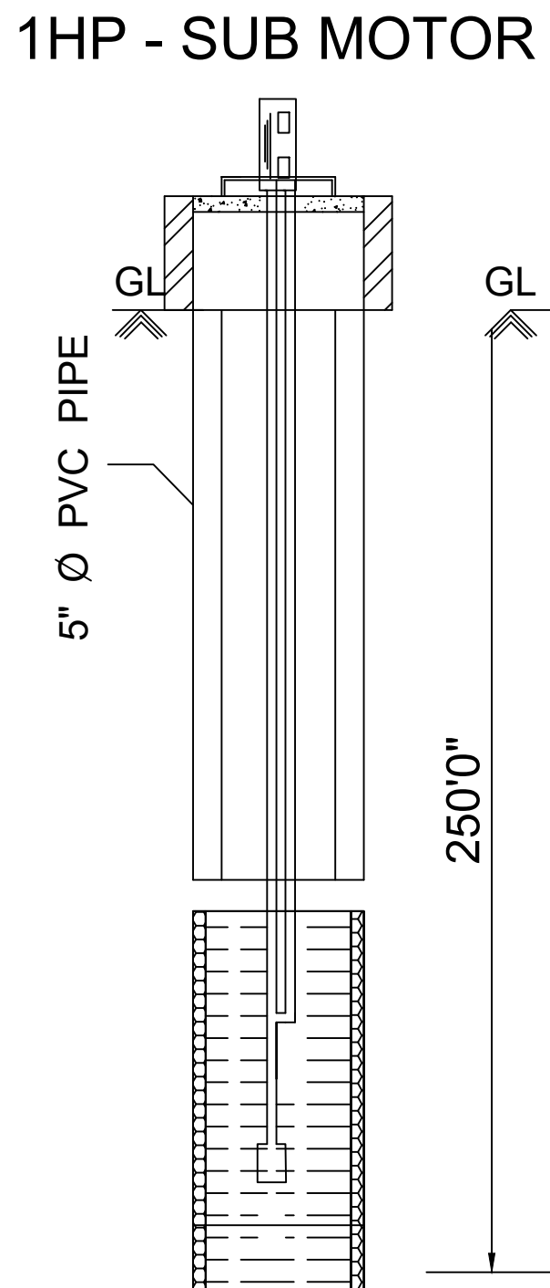
BOREWELL DETAILS
