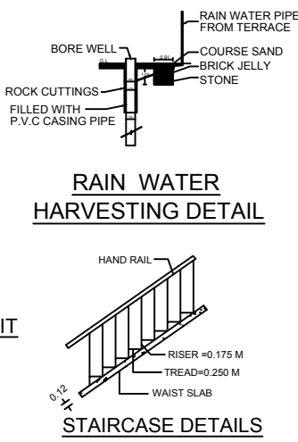
STAIRCASE DETAILS
