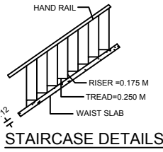
STAIRCASE DETAILS
