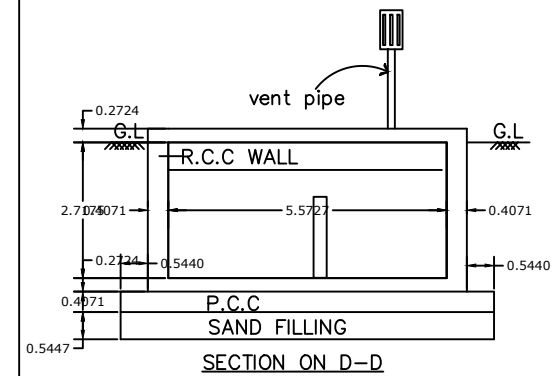
SECTION ON D-D
