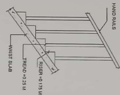
STAIR CASE DETAILS
