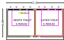
TOILET BLOCK
