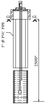
BOREWELL DETAILS
