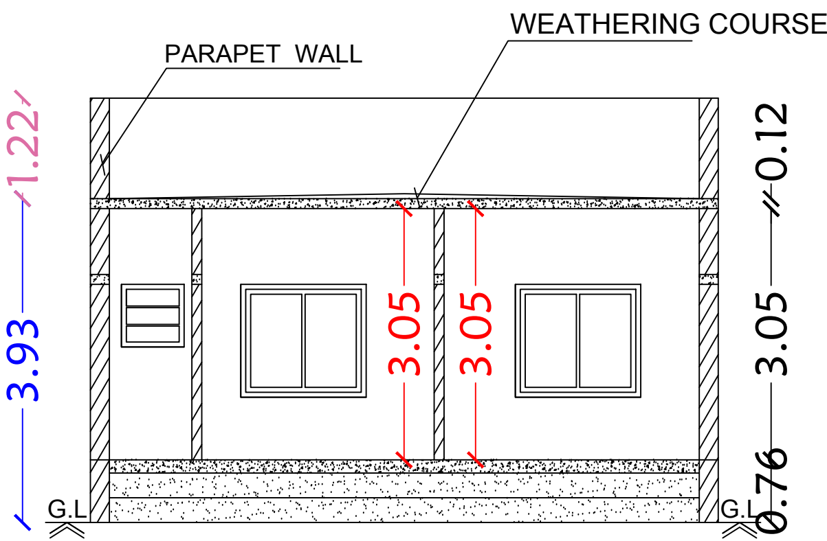
Section on-"AA"
