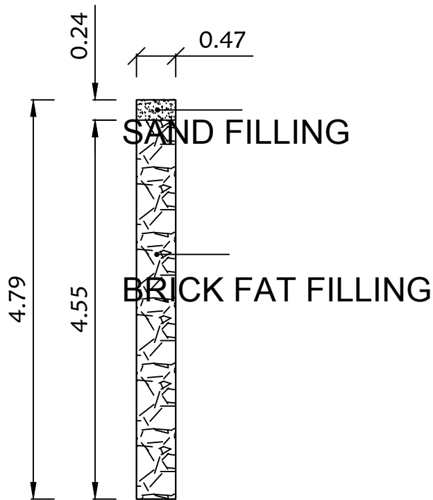
DETAILS OF PERCULATION PIT
