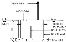
SECTION OF SEP.TANK
