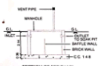
SECTION OF SEPT TANK
