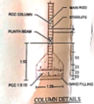
COLUMN DETAILS
