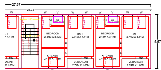
ND FLOOR PLAN
