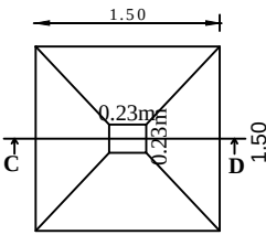
SECTION - 'CD'
