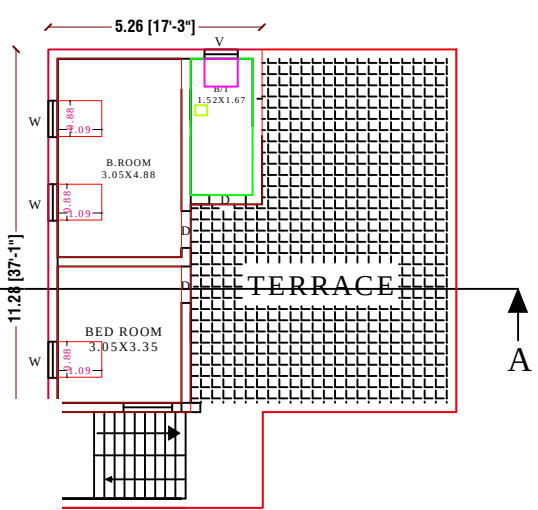
RO.FIRST FLOOR PLAN
